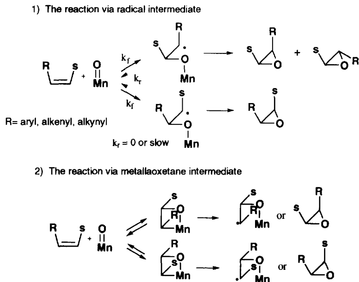
Scheme 3
