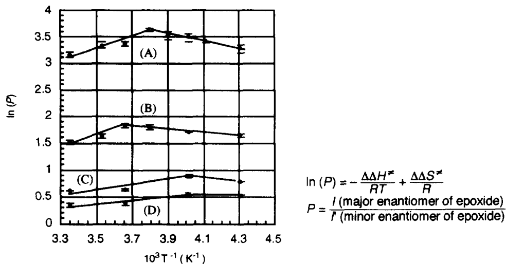
Fig. 2. Temperature dependence of enantioselectivity in the epoxidation with 3a as a catalyst. The reaction was carried out in acetonitrile in the presence of pyridine N -oxide. The enantioselectivity of the obtained epoxides was determined by HPLC or GLC analysis using optically active column or by ^1\text{H} NMR analysis using chiral shift reagent (see experimental section). The lines (A, B, C, and D) stand for dihydronaphthalene, cyclooctadiene, p -nitrostyrene, and styrene, respectively. The average \ln(P) value at each measurement point is marked with a black dot. The bars above and below the dot mean the obtained highest and lowest values of \ln(P) , respectively.
