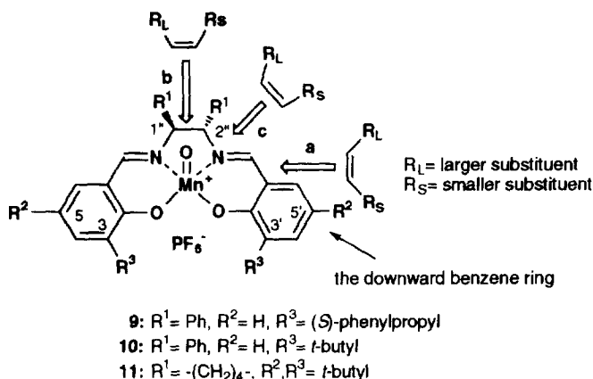
Fig. 3 The oxo Mn-salen complexes derived from the corresponding Mn-salen complexes ( 9 , 10 , and 11 ) and the proposed pathway for olefin's access
