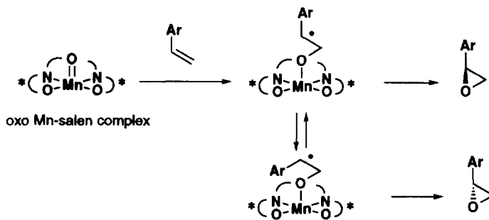
Scheme 4
