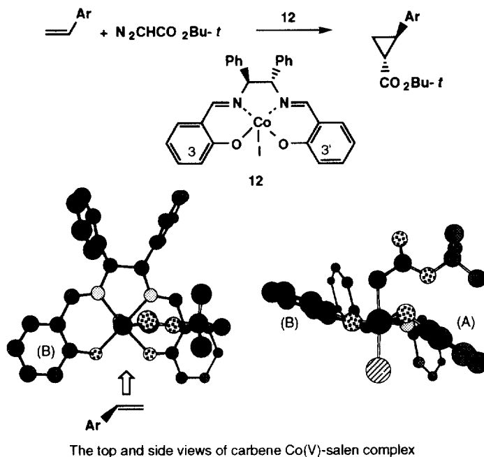
Scheme 7
