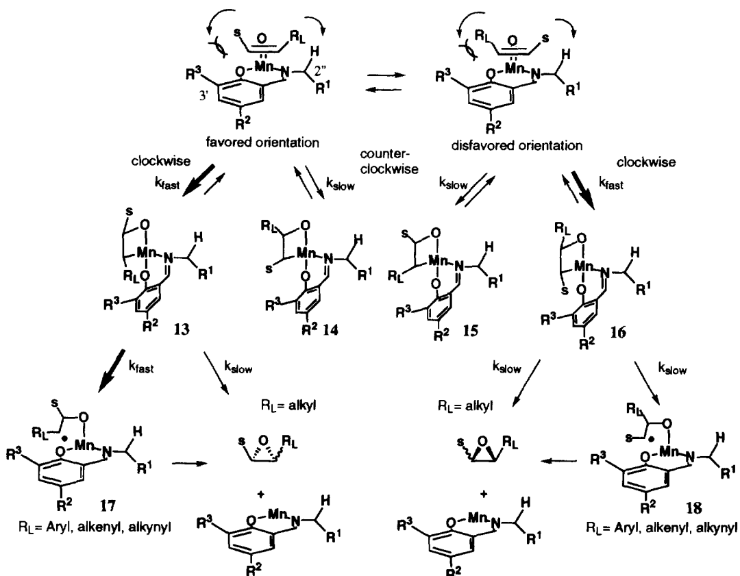
Scheme 8 The oxo Mn-salen complex is viewed from the downward benzene side (see, Fig. 3) and its backhalf is omitted for clarification. Donor ligand attached to Mn-salen and oxo Mn-salen complexes are also omitted for clarification.
